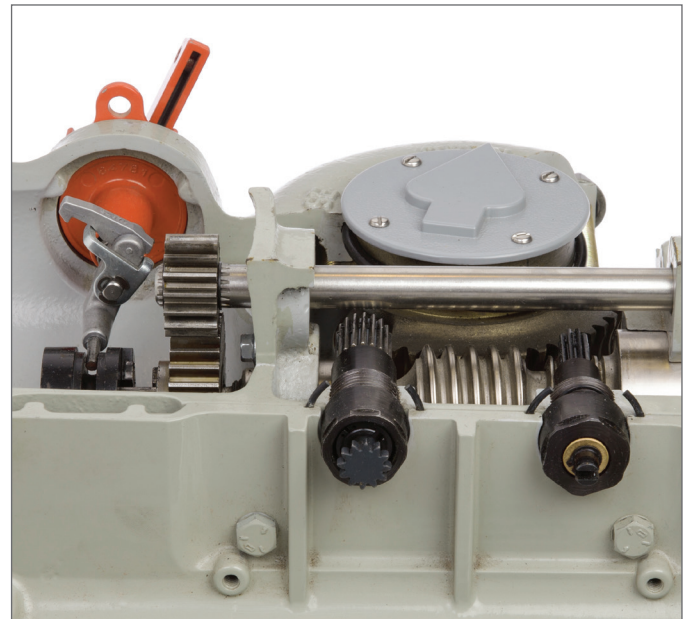
Drive assembly cutaway view
