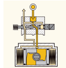
Coil Energized
