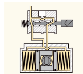
Coil de-energized
