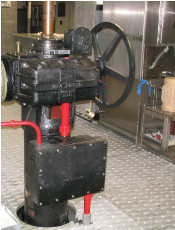
Current M2CP units evolved from proven technology—as shown by this Bettis actuator, still operating after more than 50 years at a water distribution and storage system in New York City.
