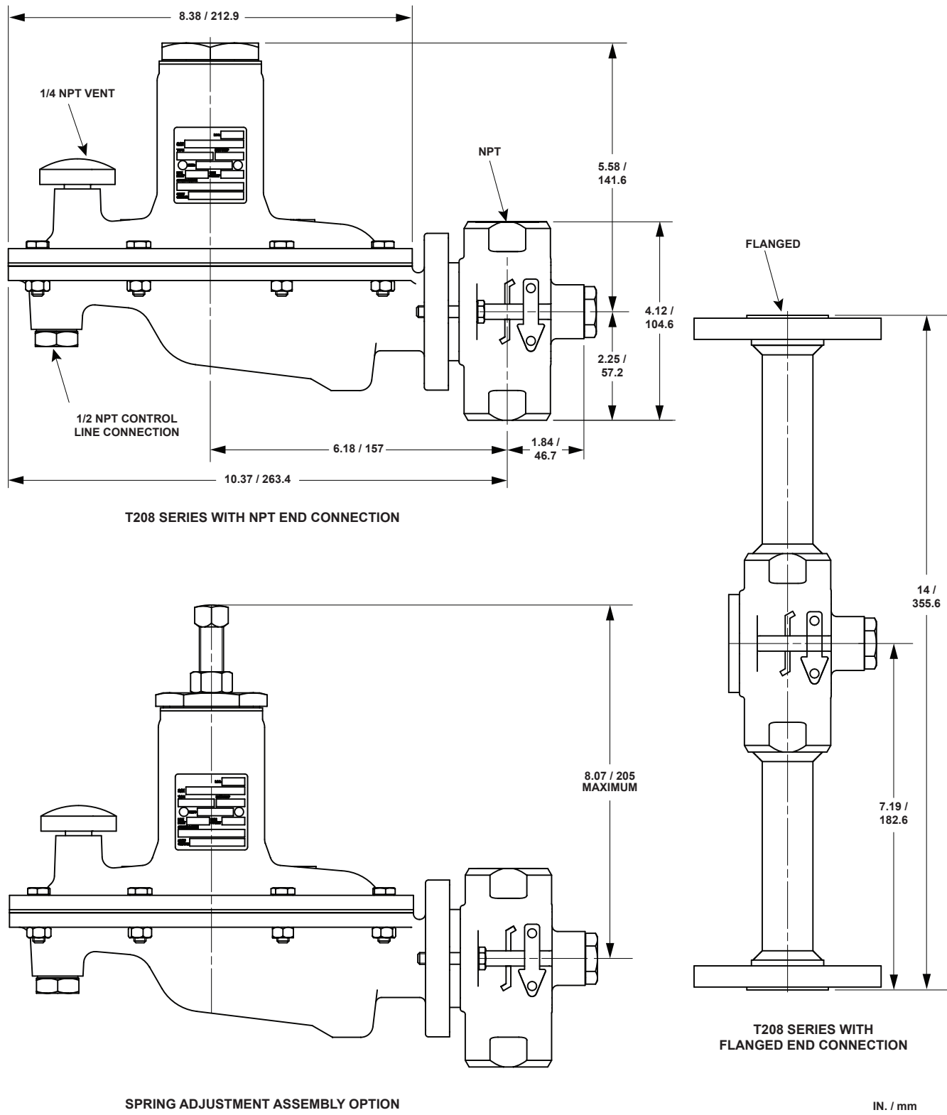
Figure 5. Dimensions
