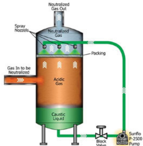
Figure 1. Typical Gas Scrubber
