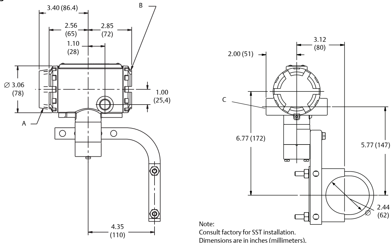
Figure 8. Remote Mount Transmitters
