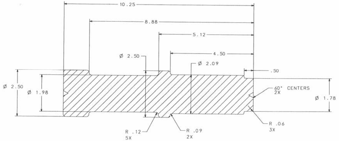
CFR / ETFE Drive Lug Disassembly Tool (PT0820) Material: UHMW Fig. 11-8
