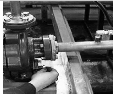
Fig. 7-2: Casing Drain
