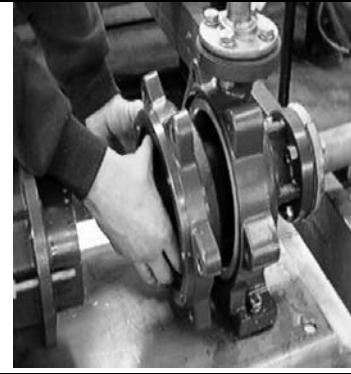
Fig. 7-8: Remove Rear Support
