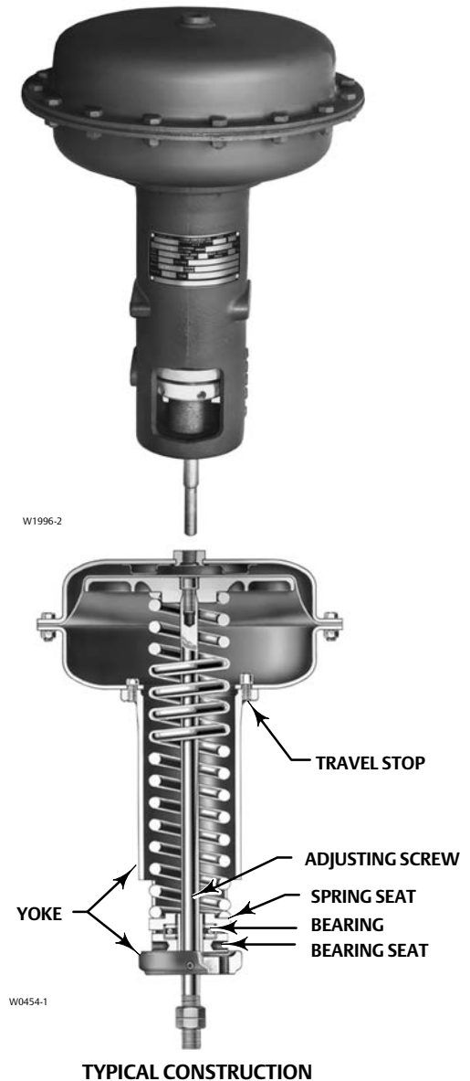
TYPICAL CONSTRUCTION
