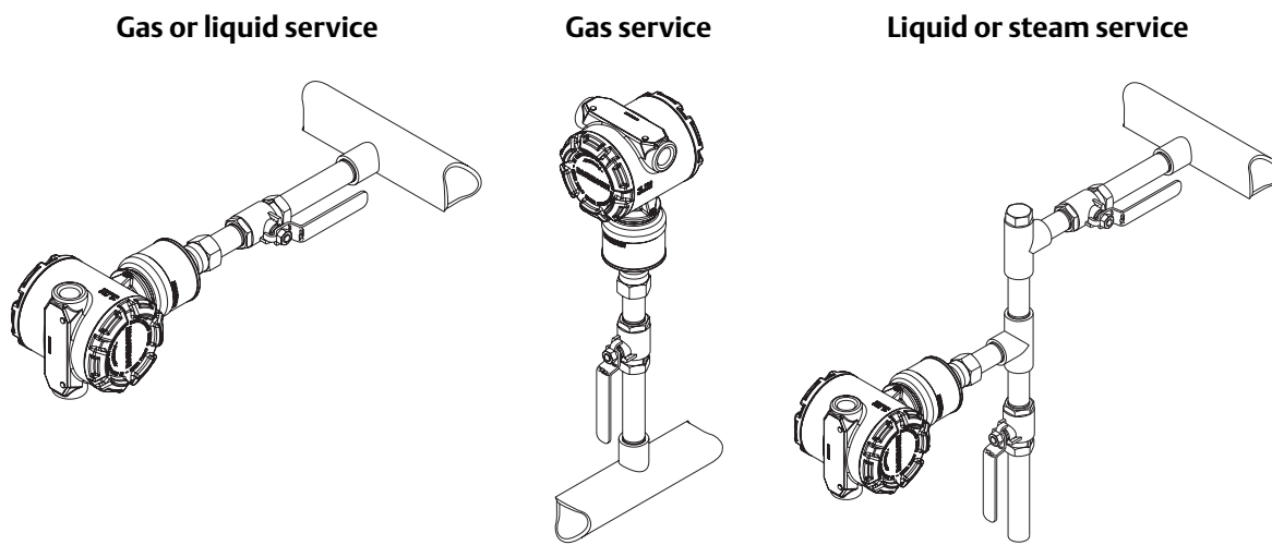
Figure 2-5. In-Line Installation Examples
