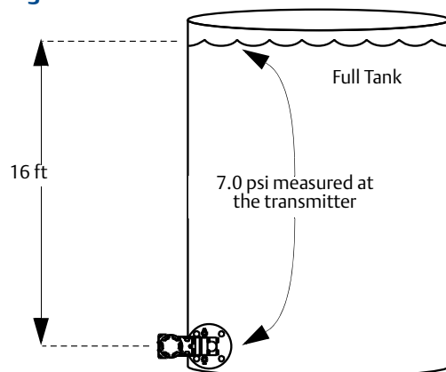
Figure 3-1. Tank Level
