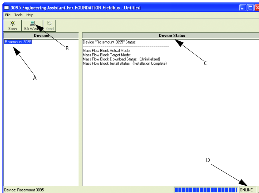
Figure 3-6. Device View
