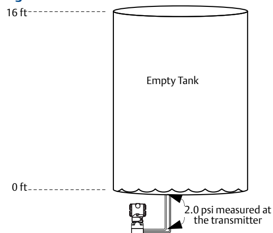
Figure 3-2. Tank Level
