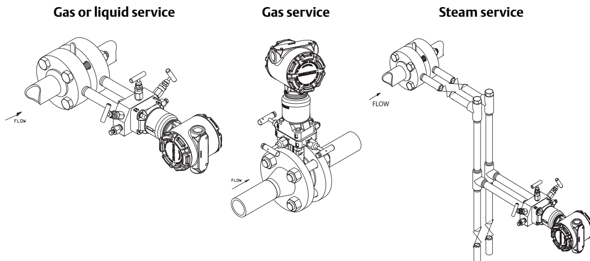
Figure 2-4. Coplanar Installation Examples
