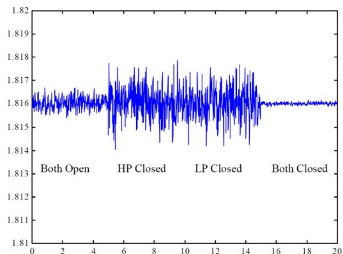
Figure 6-17. Differential Pressure Signals under Different Plugging Conditions
