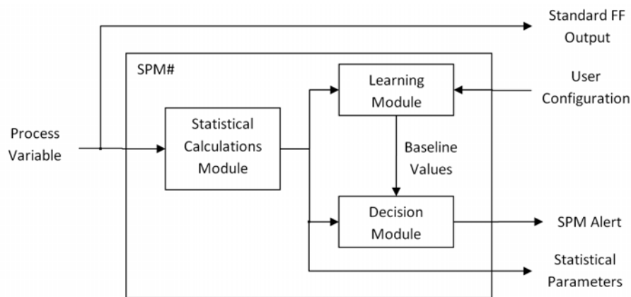
Figure 6-3. Rosemount 3051S FF Statistical Process Monitoring
