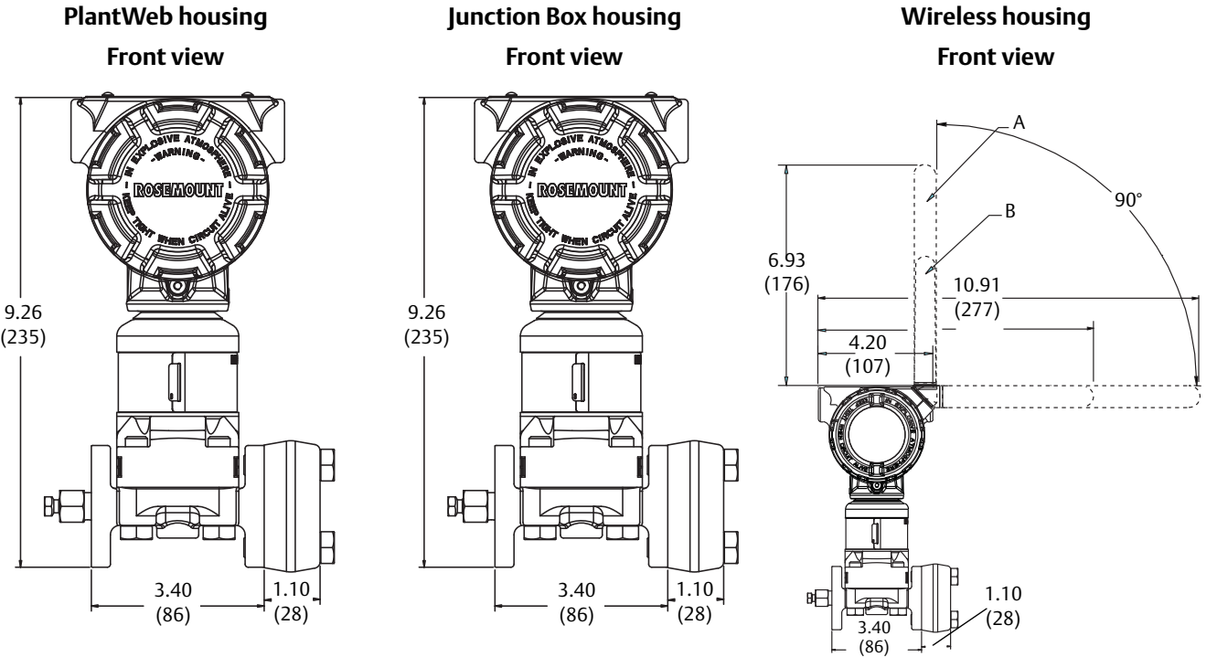
Figure A-2. Transmitter with Coplanar Sensor Module and Traditional Flange
