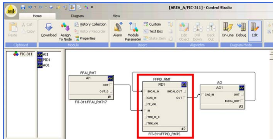
Figure 6-9. Example of PID Control within a Pressure Transmitter
