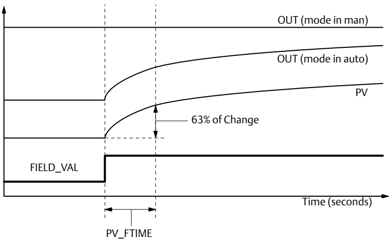
Figure 3-3. Analog Input PV_FTIME filtering
