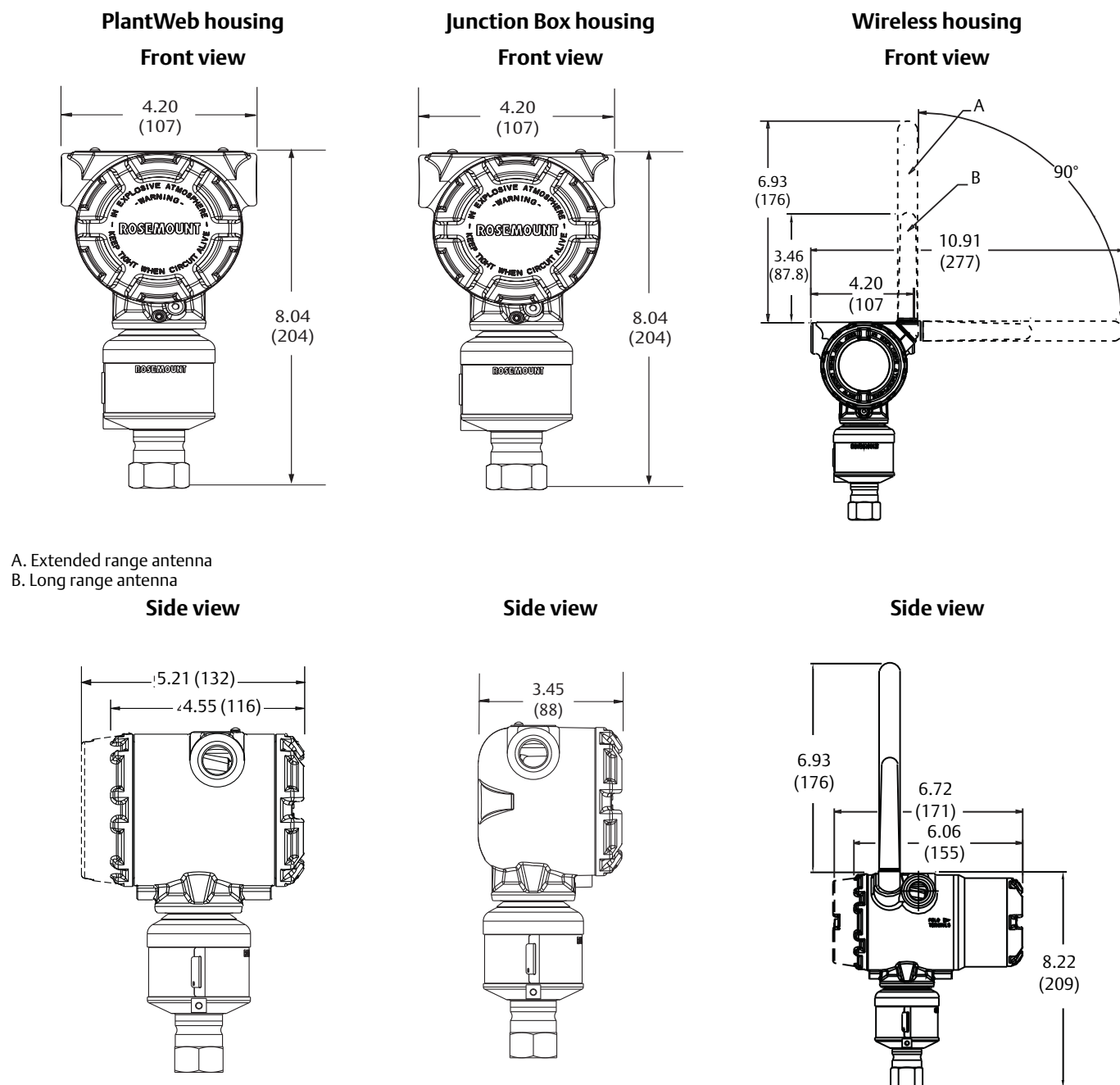
Figure A-3. Transmitter with In-Line Sensor Module
