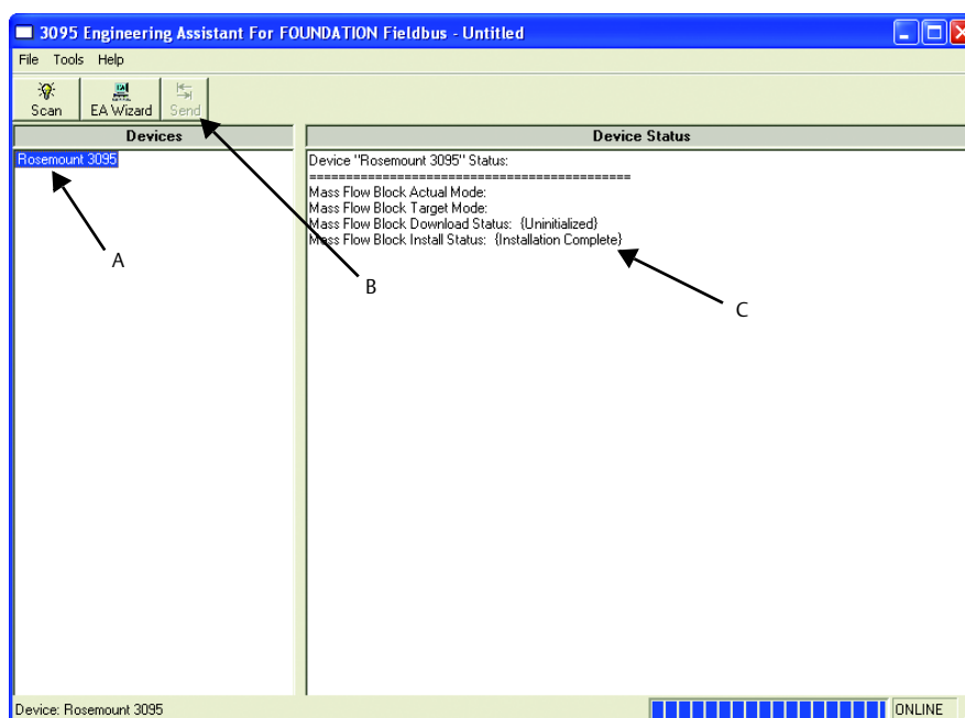
Figure 3-9. Download Mass Flow Configuration File
