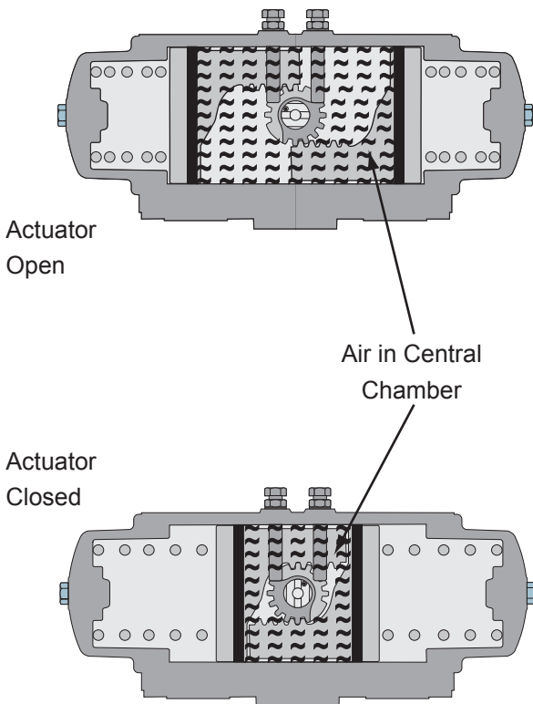
Spring Return and Double Acting Actuators
