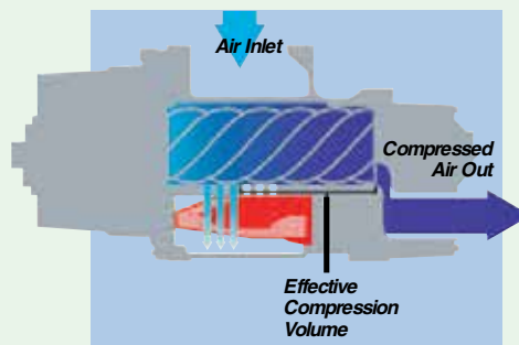
PARTIALLY OPEN BYPASS PORTS
